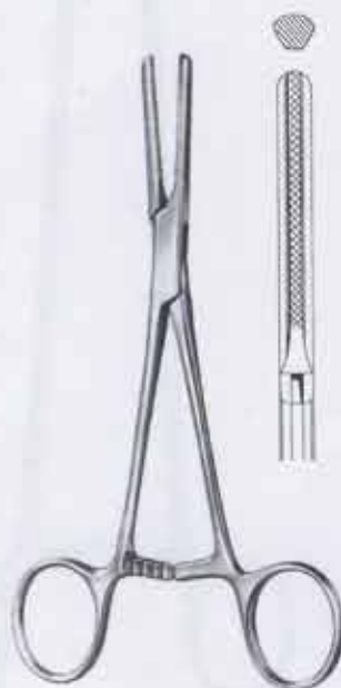
HF.3944.15 15.5 cm/6" HF.3944.19 19.0 cm/7½" HF.3944.20 20.5 cm/8"
